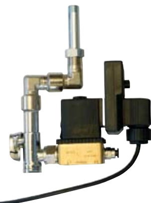
Assembly of the automatic drainage with timer (optional) COPURA-LUX
