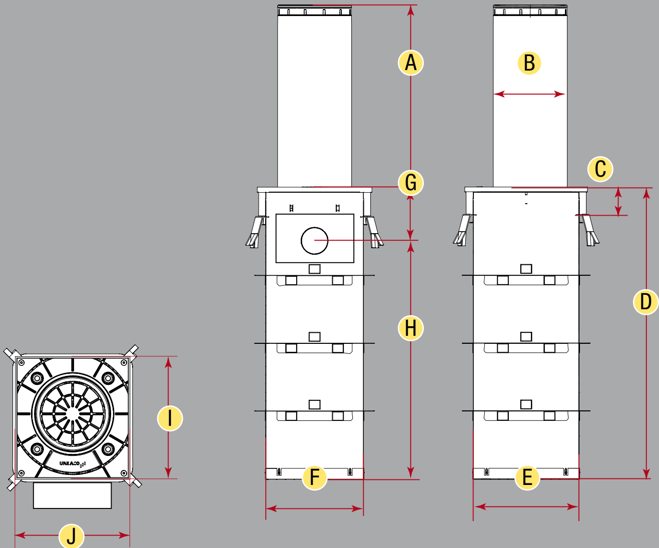
DIMENSIONS OF THE BOLLARD (see drawing)
